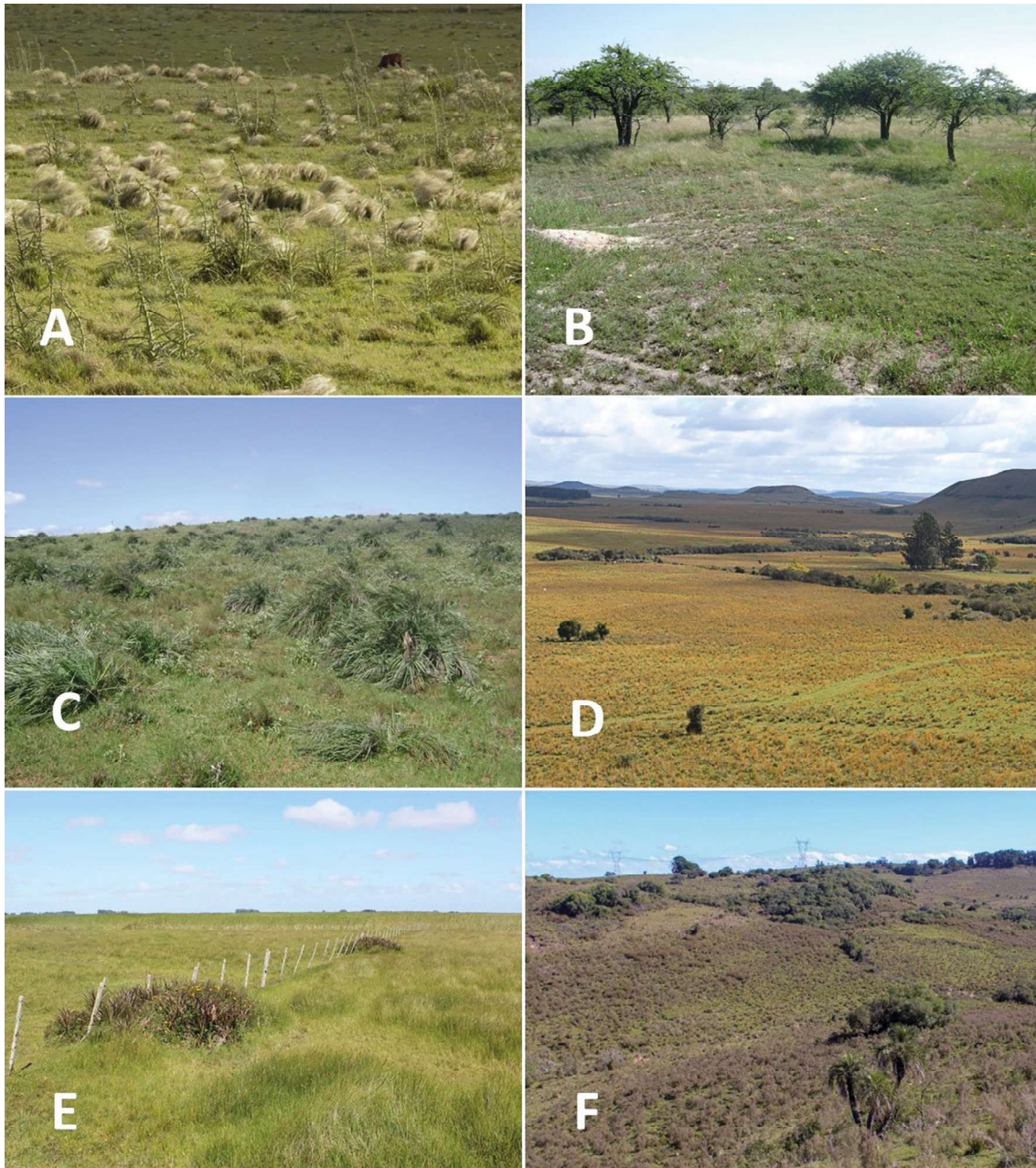
Figure 3-A. Ecoregions and characteristic physiognomies of the Pampa biome. A) Field with Jubata Grass ( Aristida jubata ), in the municipality of Júlio de Castilhos, RS; B) Field with Espinilho ( Vachellia caven ), in Espinilho State Park, in the municipality of Barra do Quaraí, RS; C) Sandy Field, dotted with Dwarf Palm ( Butia lallemantii ), in the municipality of Manoel Viana, RS; D) Mixed Field with Andropogoneae and Compositae, in the municipality of Rosário do Sul, RS; E) Coastal Field, in the municipality of Rio Grande, RS; F) Shrubland, in the municipality of Pinheiro Machado, RS.
