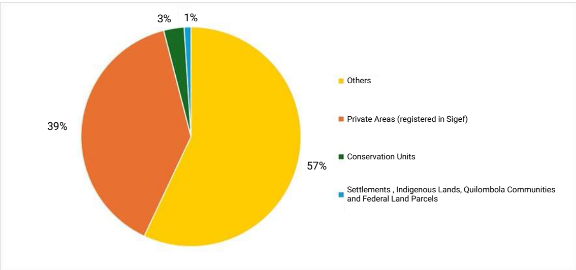
Figure 12. Distribution of land title categories in the Pampa biome in 2023.
