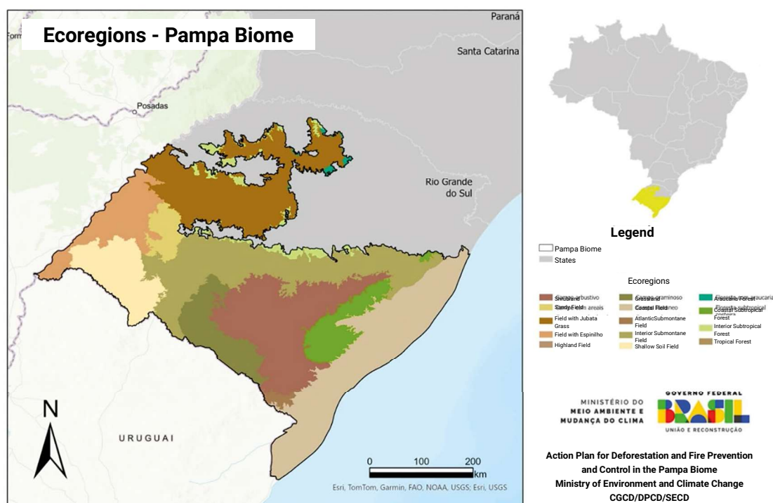
Figure 2. Ecoregions of the Pampa biome.
