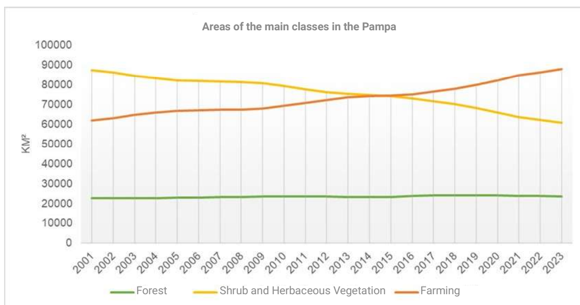
Figure 10. Areas of the main classes in the Pampa biome between 2001 and 2023.
