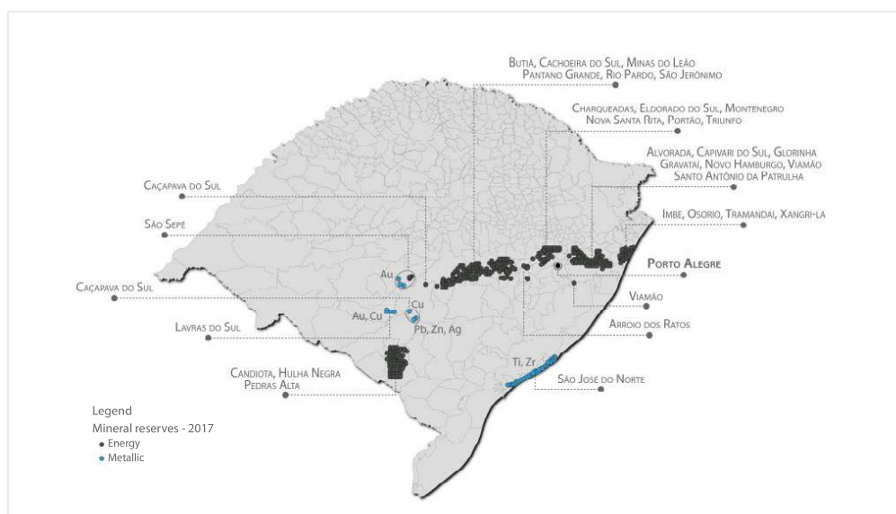
Figure 23. Location of metallic and coal reserves in Rio Grande do Sul.
